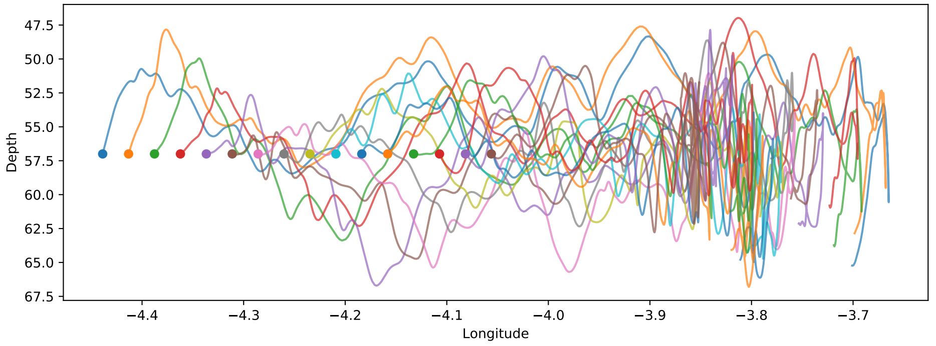
Lon vs z
