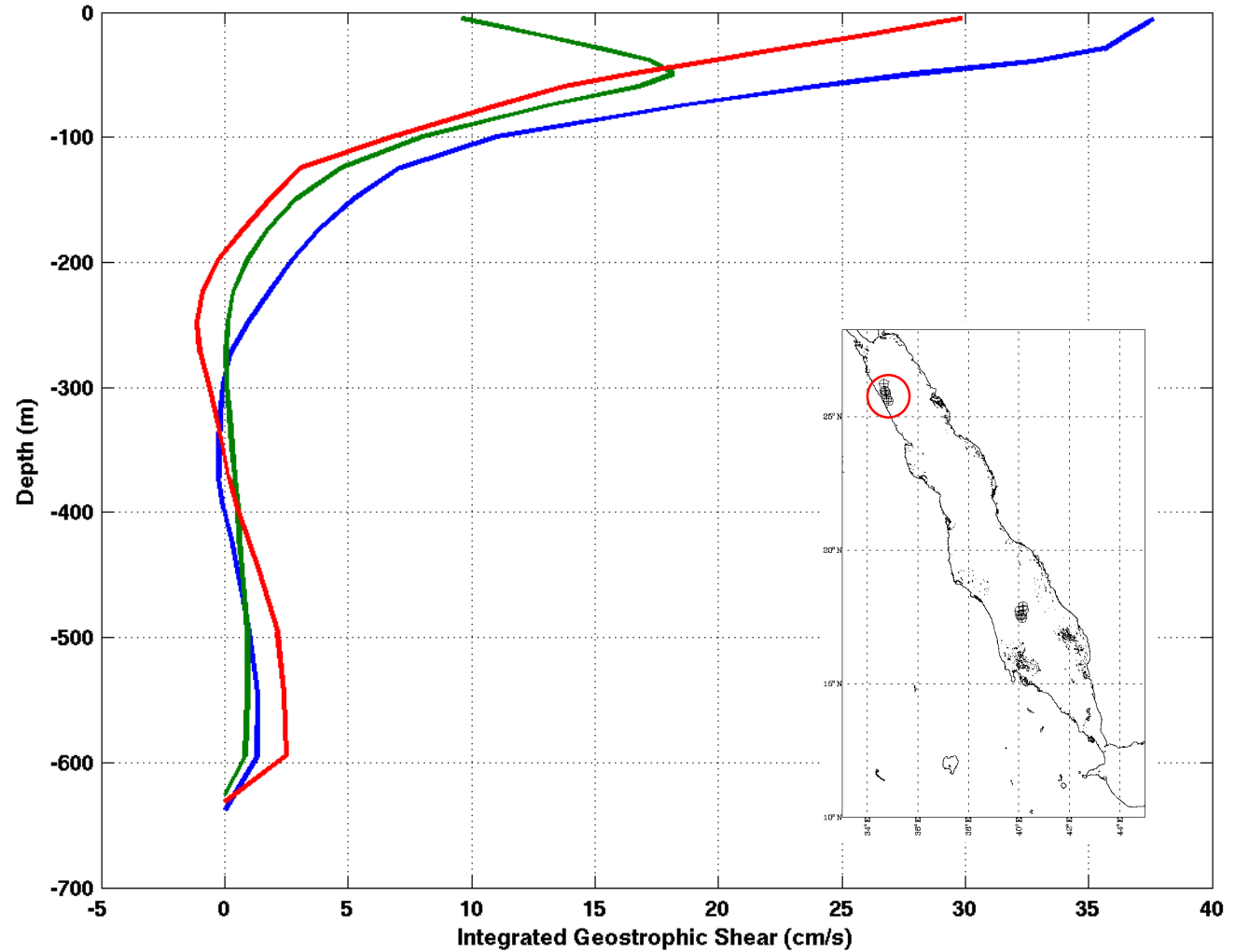
Density currents (estimated from GTSP 2000 data)
