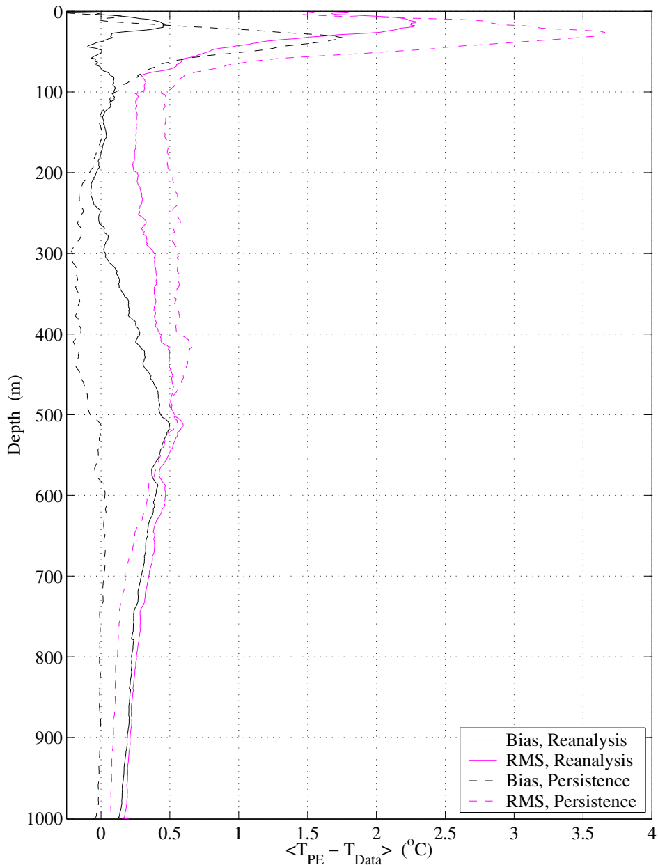
Fig. 16. Reanalysis Temperature Bias ( ^{\circ}\text{C} ) and RMS ( ^{\circ}\text{C} ) comparisons, averaged over Aug 21-25. In this reanalysis simulation, only data up to Aug 20 was assimilated. Persistence is defined as the Aug 20 objective analysis of all data up to Aug 20.
