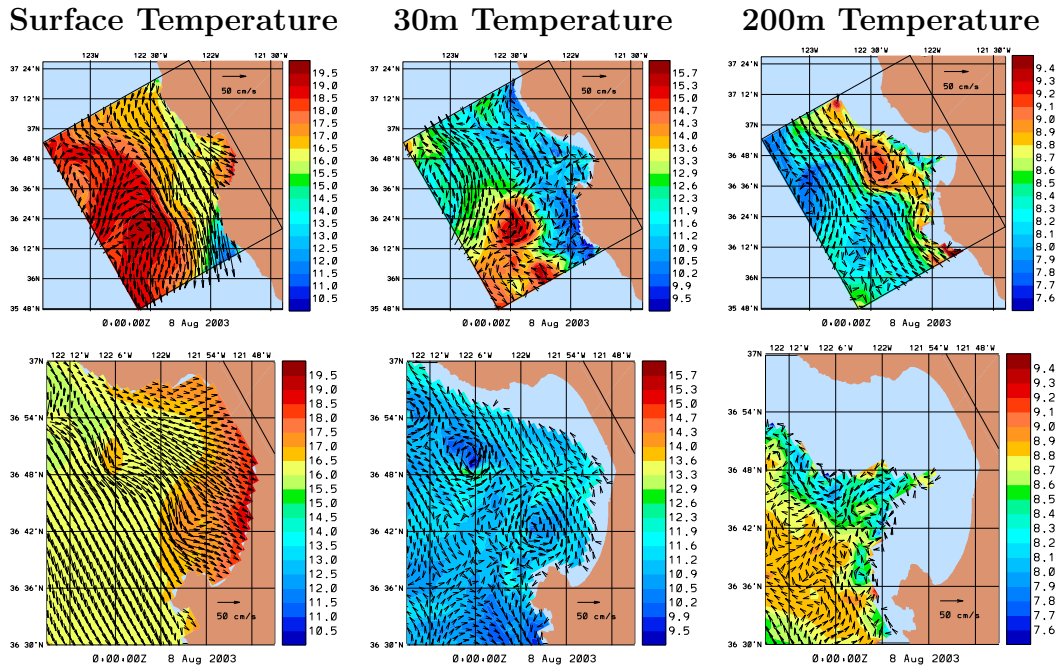
Fig. 5. Temperature ( ^{\circ}\text{C} ) and velocity ( \text{cm/s} ) fields for Aug 8, 2003 issued during the real-time exercise. These fields show the general structures that were observed in real-time.
