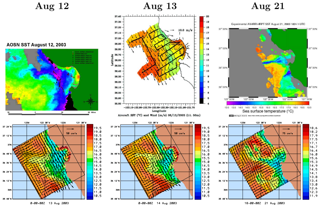
Fig. 7. Comparisons of (top row) available real-time SST ( ^{\circ}\text{C} ) images from satellite (Aug 12 and 21) and aircraft (Aug 13) with (bottom row) corresponding real-time forecast surface temperature ( ^{\circ}\text{C} ) fields. Note timing conventions (e.g. 0000Z 13 Aug forecast corresponds to 1600 local 12 Aug and is compared to 12 Aug image).
