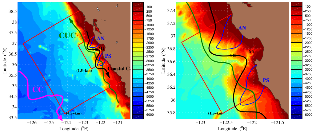
Fig. 1. Modeling domains for AOSN-II with bathymetry. Left panel shows the “Data Domain” inside of the larger “Offshore Domain”. Right panel shows a zoom of the “Data Domain”. Also shown are the main dynamical features: upwelling centers at Point Año Nuevo (AN) and Point Sur (PS) (blue); coastal current, eddies, filaments, etc. (black); California Undercurrent (CUC) (green); California Current (CC) (magenta).
