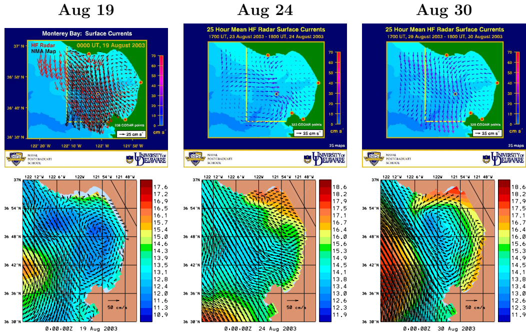
Fig. 8. Comparisons of (top row) available real-time CODAR (cm/s) images with (bottom row) corresponding real-time forecast surface velocity (cm/s) fields.
