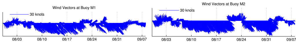
Fig. 2. Wind vectors (knots) at the M1 and M2 moorings.
