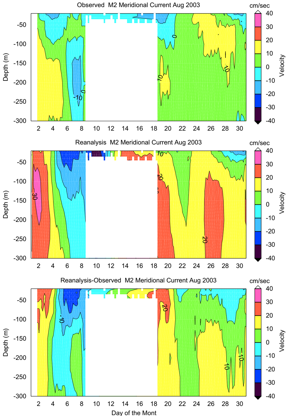
Fig. 21. The same as Fig. 19 except at the M2 location.
