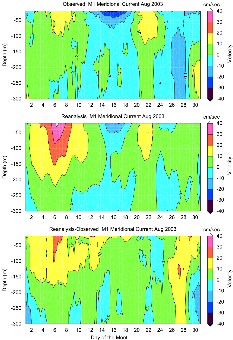
Fig. 19. The same as Fig. 18, except for meridional current.
