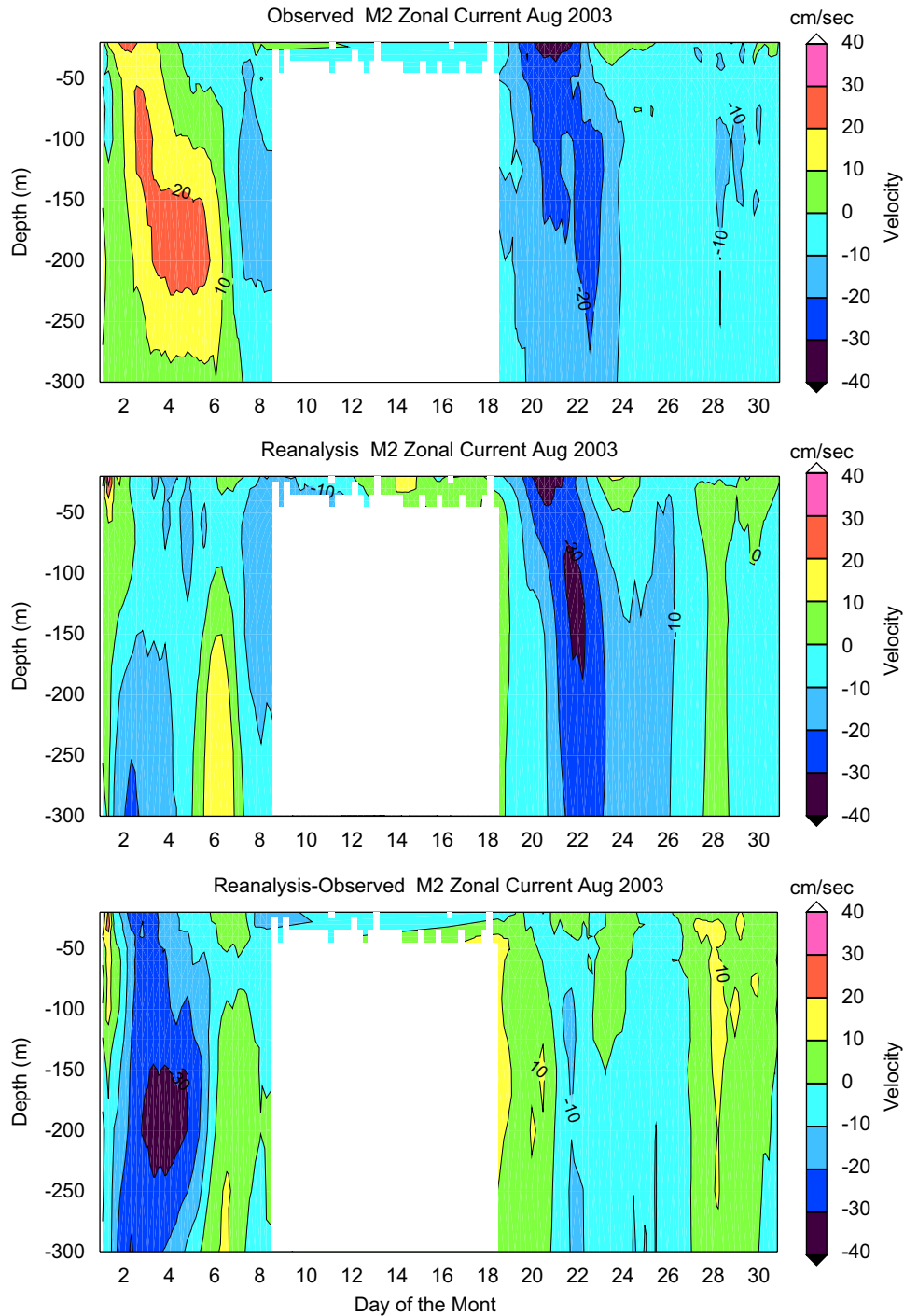
Fig. 20. The same as Fig. 10 except at the M2 location.
