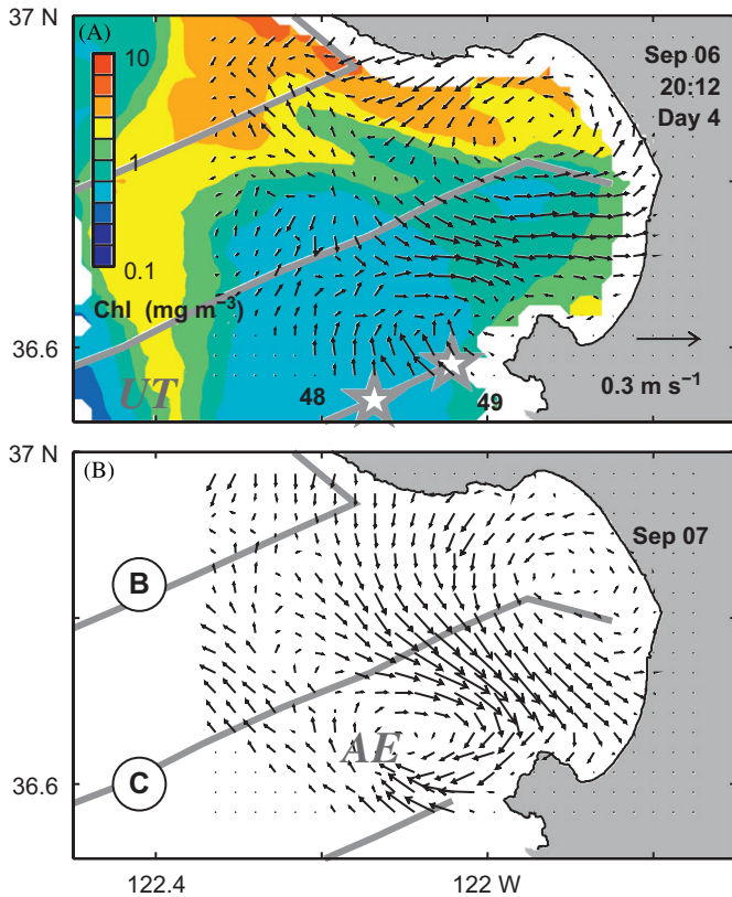
Fig. 10. The CODAR daily mean surface currents from (A) cruise day 4 and (B) one day after the cruise (7 September 2003) are superimposed on sea-surface chlorophyll from SeaWiFS. The upwelling tongue (UT) is labeled (Section 4.3). Dates and times are UTC. Gray lines show transects B–D and gray stars in (A) indicate thin layers were found on the flanks of the developing anticyclonic eddy (AE) at stations 48 and 49 on cruise day 4.
