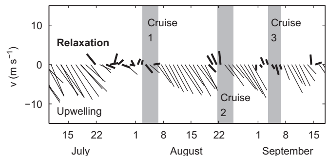
Fig. 2. Daily mean wind vectors measured at the MBARI M2 mooring near station 6 from July to September 2003. The three cruises are indicated by gray shading. Upwelling-favorable winds are southward. Vectors show the direction towards which the wind is blowing (north is up, east is right). Relaxation from upwelling conditions is defined as southward winds with speeds < 3 \text{ m s}^{-1} or northward winds. Relaxed winds are denoted by bold vectors.
