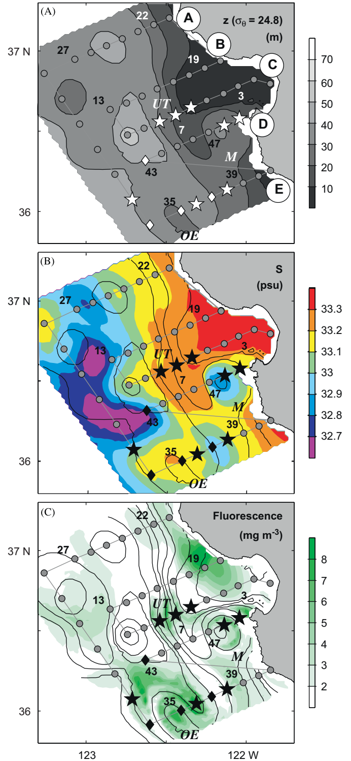
Fig. 13. (A) Depths of the \sigma_\theta = 24.8 kg m -3 isopycnal for cruise 3 are plotted and contoured (black) in 10- and 5-m intervals in (B) and (C). (B) Salinity and (C) fluorescence are plotted on \sigma_\theta = 24.8 kg m -3 . Gray dots indicate CTD stations, stars indicate thin layer locations, and diamonds indicate nearby subsurface chlorophyll maxima. The upwelling tongue (UT), meander (M), and offshore eddy (OE) are labeled (Section 4.3).
