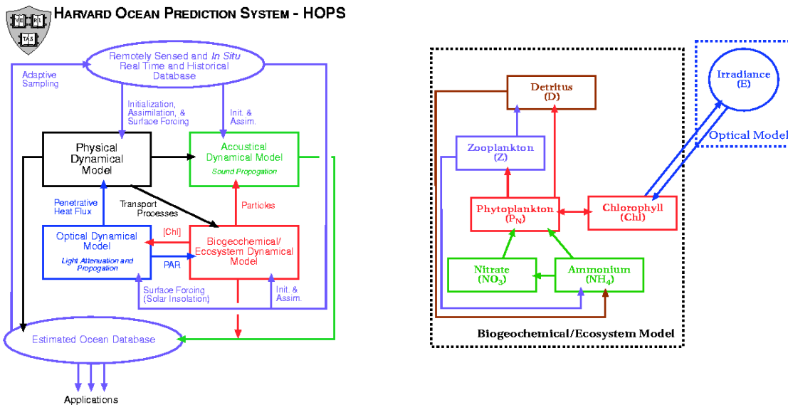
Figure 2 - HOPS system schematics. a) overall HOPS system, b) biogeochemical/ecosystem model
