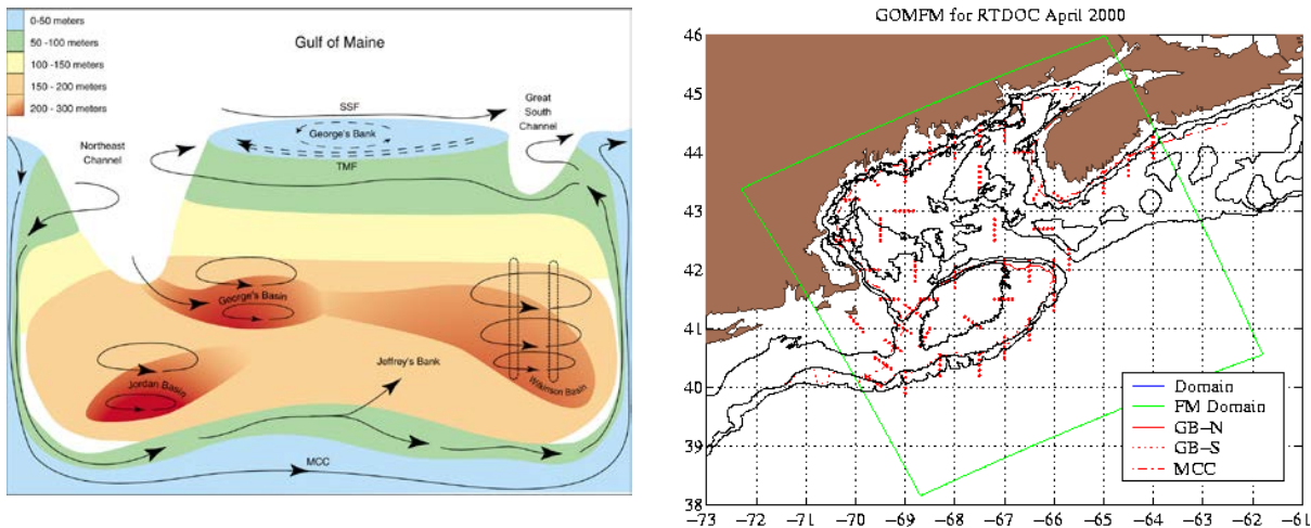
Fig. 4. a) A 3-D perspective of the circulation of the Gulf of Maine/Georges Bank system. The selected features of the coastal circulation system are shown overlaid on preferred topographic regions. The blue band signifies the 0-50m region, the green depicts 50-100m depths, the yellow band covers the 100-150m levels, the orange covers the 150-200m deep interior regions and the red regions are the 200-300m deep basins. MCC = Maine Coastal Current, TMF = Tidal Mixing Front, SSF = Shelf-Slope Front. b) A sampling strategy for the features model initialization scheme. Temperature and salinity profiles are sampled along and across the important features of circulation and then melded in background climatology for generating coastal ocean field. The coastal fields are then melded with the deep (GSMR) fields via the shelf-slope front to yield the initialization for the AFMIS simulations.
