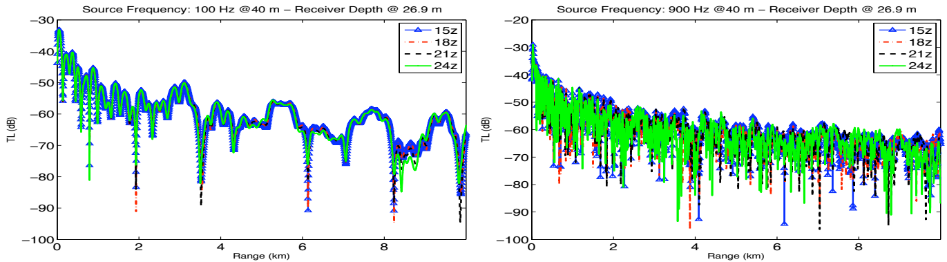
FIGURE 9. Acoustic TL prediction in the along Dabob Bay section for 100 and 900 Hz source at depth of 40 m, and receiver depth of 26.9 m. Four different color lines in the each panel indicate the TL prediction in one section at four different times during one tidal period.
