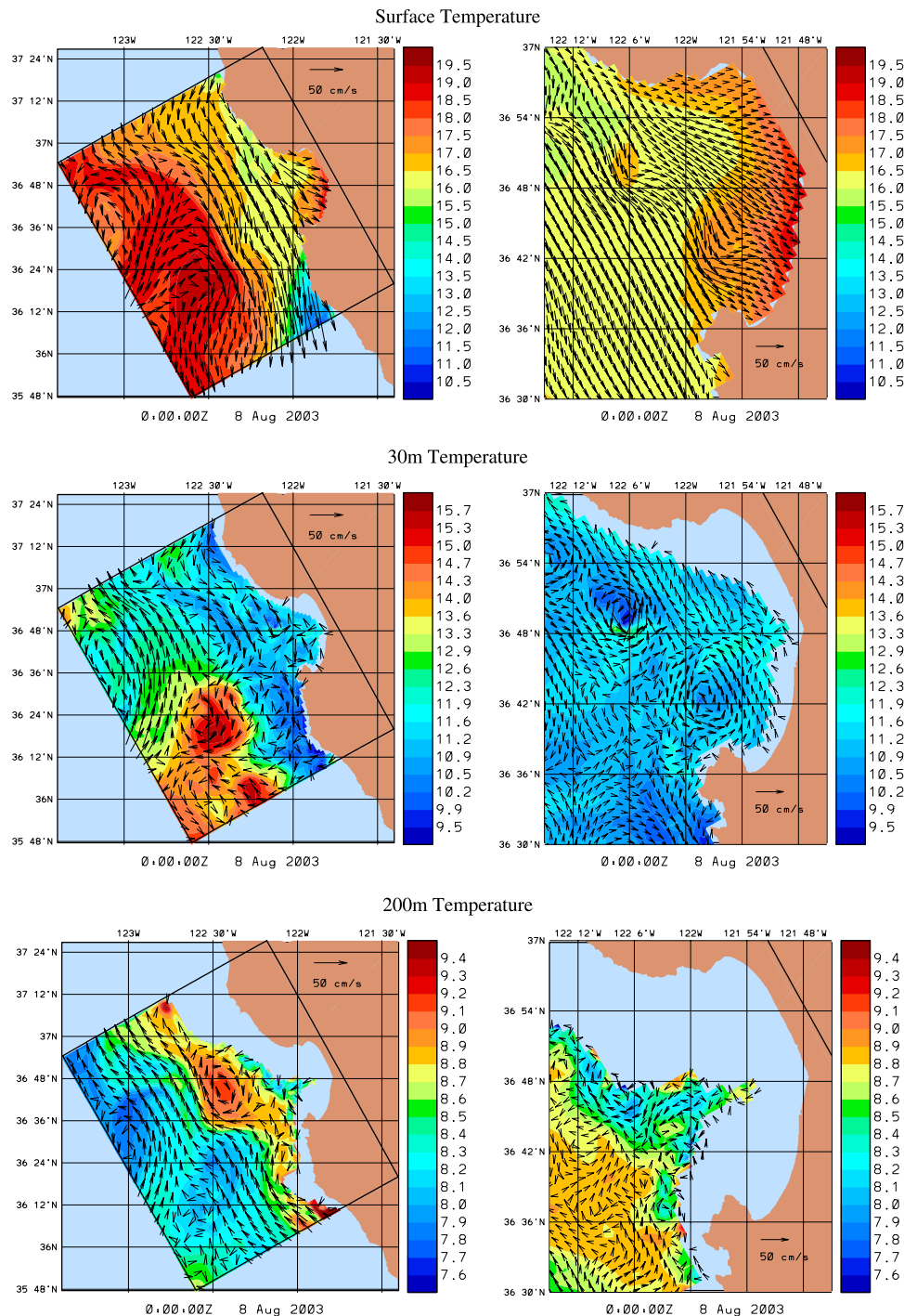
Fig. 5. Temperature (°C) and velocity (cm/s) fields for August 8, 2003 issued during the real-time exercise. These fields show the general structures that were observed in real-time.
