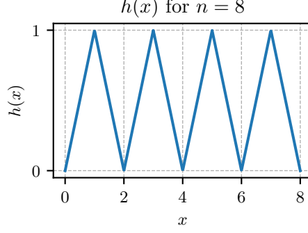
Figure 2: Sample form of function h(x) used in constructing g_{S,b}(\mathbf{A}) as a GNN. For the construction, we will have x = \sum_{i \in S} [\mathbf{c}_A]_i .
