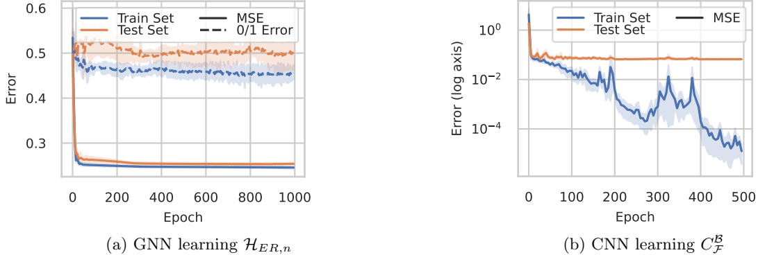
Figure 1: Overparameterized GNN (a) and CNN (b) fail to learn functions from the class \mathcal{H}_{ER,n} and C_{\mathcal{F}}^B respectively by either failing to fit the training set or overfitting the data. Plots are aggregated and averaged over five random realizations.
