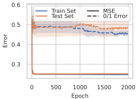
(a) GNN learning \mathcal{H}_{ER,n}
