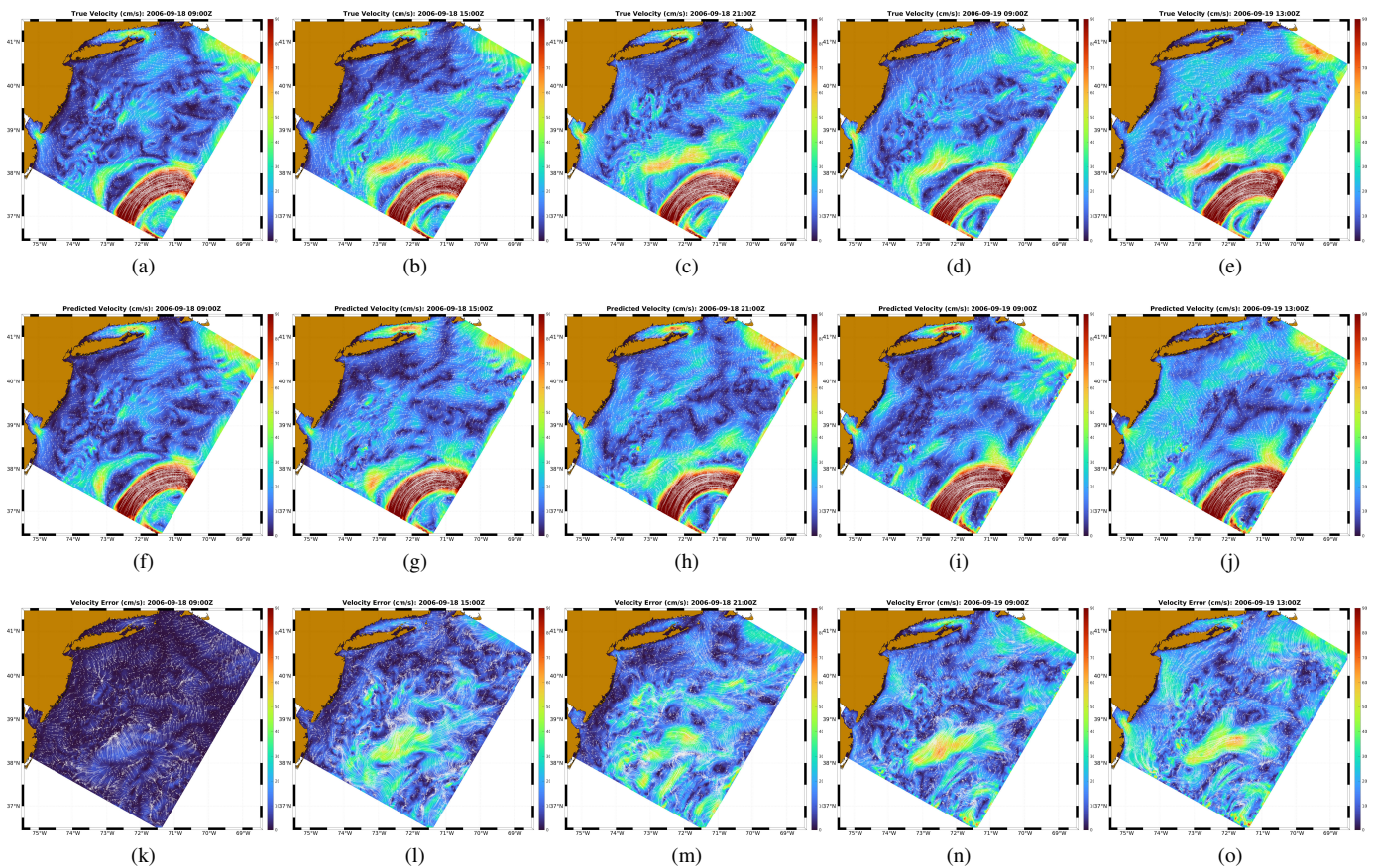
Fig. 1: Applying FCN in the MAB . Surface velocity field amplitudes overlaid with curved velocity vectors. Ground truth from the MSEAS-PE forecast (top row), FCN predictions for training-run 246 (middle row), and error fields (bottom row) for five different forecast times: 2006 Sep 18 09Z and 6, 12, 24, and 28 hours later.
