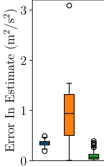
Figure 12: Absolute error in estimating (approximate) test risk in the wind speed experiment for the holdout (blue), 1NN (orange) and our SNN (green). It appears that SNN has the smallest error in estimating the ground truth, although the approximate ground truth we compute via Monte Carlo estimate is not entirely theoretically justified. However, due to the relatively large differences across most seeds, we still expect the difference is indicative of better performance of SNN.
