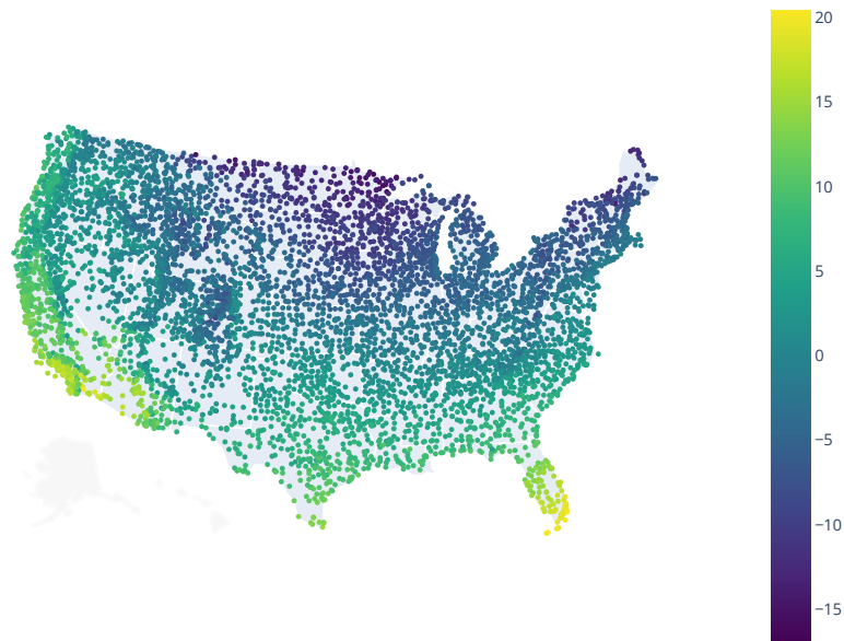
Figure 8: Weather stations used in the air temperature prediction task we considered, colored by average temperature in January 2018 in degrees Celsius.
